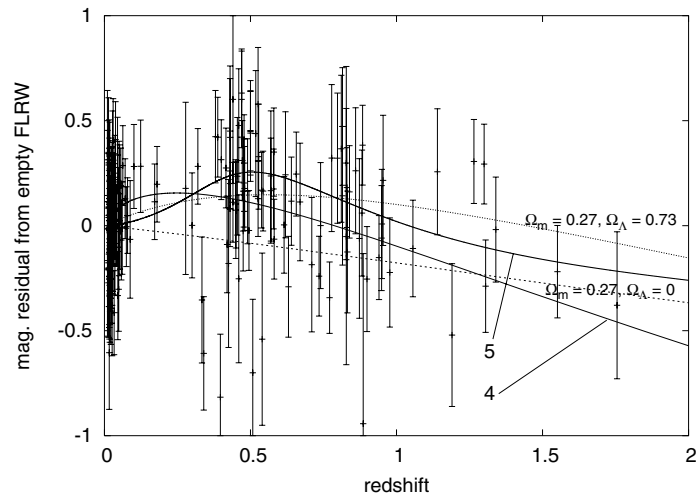
Figure 3 The residual Hubble diagram for models 4 and 5.
