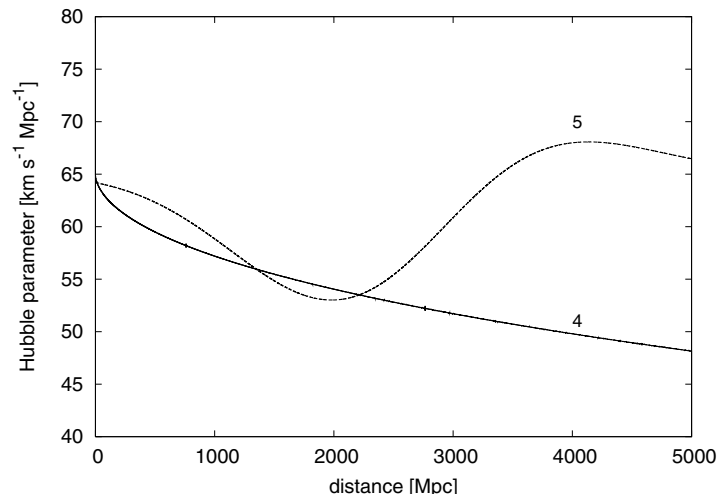
Figure 4 The Hubble parameter for models 4 and 5.
